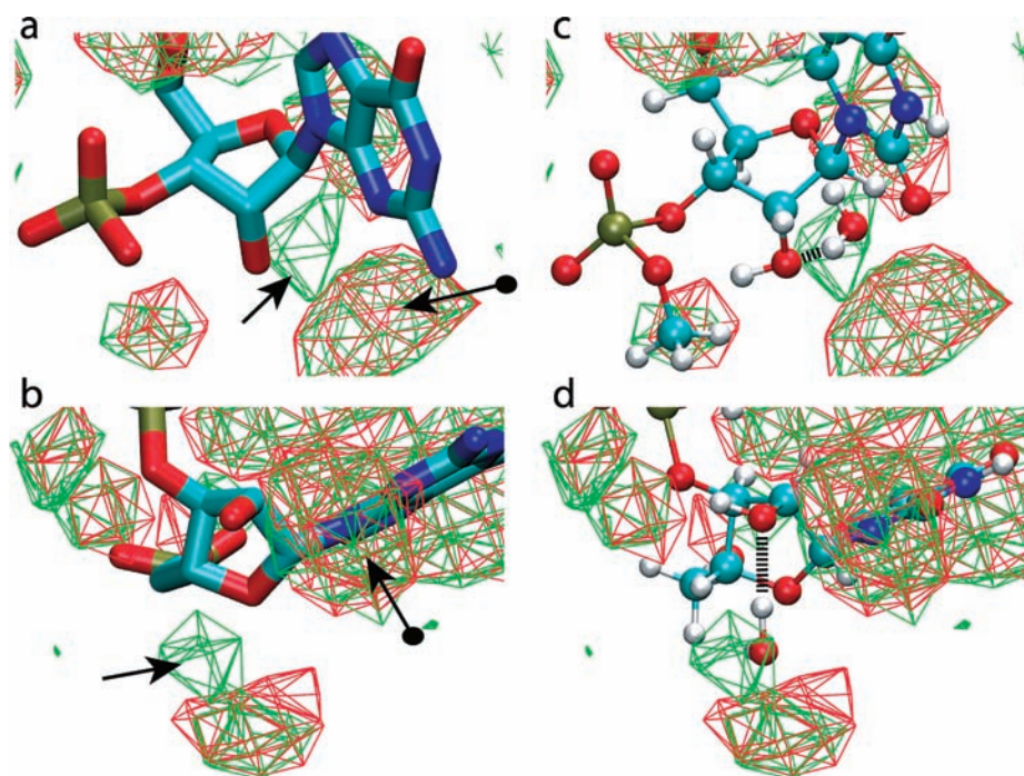
Figure 4. 3D water oxygen probability distributions around RNA nucleotides from the crystallographic survey. (a,b) Approximately orthogonal images of water distributions from canonical (red) and noncanonical (green) RNA structures. Water contour levels are at 33% occupancy and a guanine base is shown for reference although all bases were included in the survey. Standard arrow indicates the higher probability distribution region in the noncanonical nucleotides and the arrow with a sphere on the tail is the distribution associated with water interacting with both the O2' atom and the minor groove of the base. (c,d) Approximately orthogonal images of the uridine nucleotide (model compound NUSU) and the water obtained from the QM calculation overlaid on the water probability distributions from a and b in the identical orientation. The hydrogen bond between the water and the O2' atom is shown.
