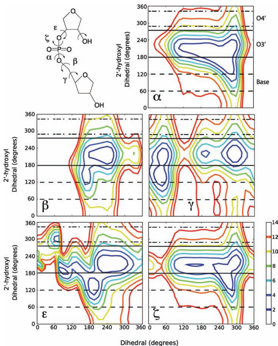
Figure 1. Model compound, R3PS, used in the QM calculations and the 2D QM potential energy surfaces (phosphodiester \alpha , \beta , \gamma , \epsilon , or \zeta torsions vs 2'-hydroxyl) for R3PS obtained at the MP2/6-31+G(d)//RIMP2/cc-pVTZ level of theory. The energy scale is in kcal/mol. The 2'-hydroxyl dihedral is defined as C1'-C2'-O2'-H2', and the three 2'-OH orientation ranges are as follow: base, 60–120° (dashed lines); O3', 190–270° (solid lines); and O4', 280–330° (dot-dashed lines).
